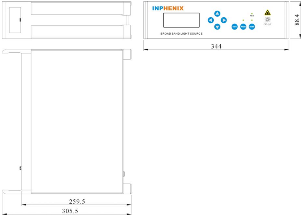
Figure 2 Mechanical drawing of IPSDM0702-xx8 SLD light source desktop
