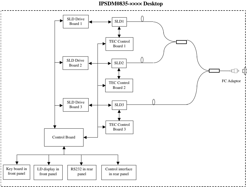
Figure 1 Configuration of IPSDM0835-xxxx SLD light source desktop
