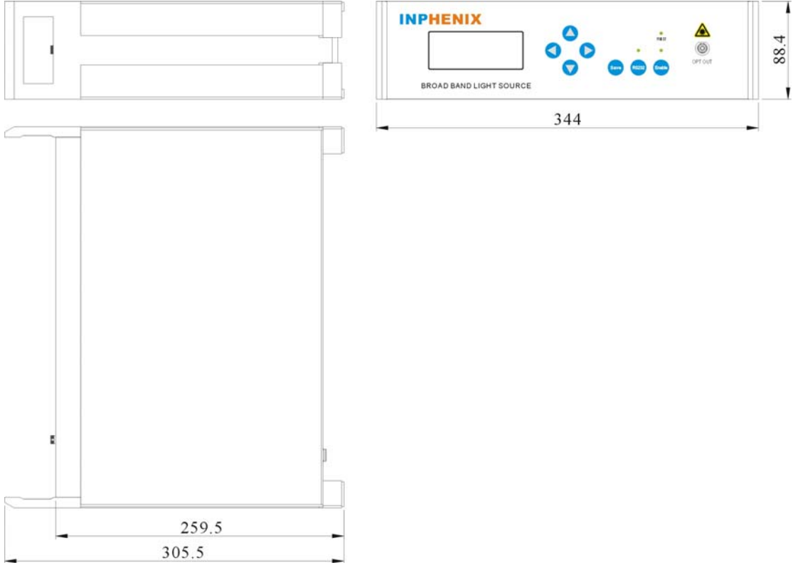
Figure 2 Mechanical drawing of IPSDM0835-0318 SLD light source desktop
