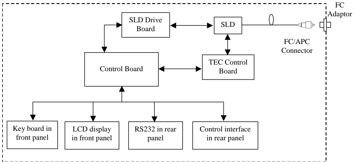
Figure 1 Configuration of IPSDM1005-xxxx SLD light source desktop
