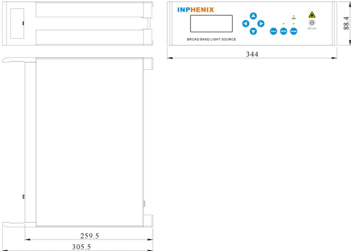
Figure 2 Mechanical drawing of IPSDM1501-xxx8 SLD light source desktop
