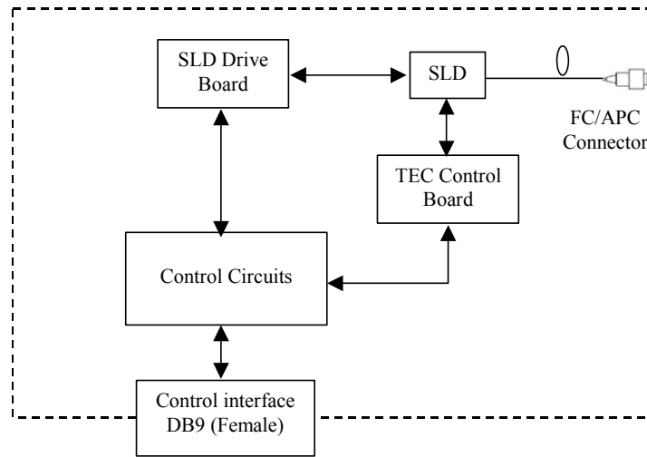
Figure 1 Configuration of IPSDS1503-xxxx SLD light source module
